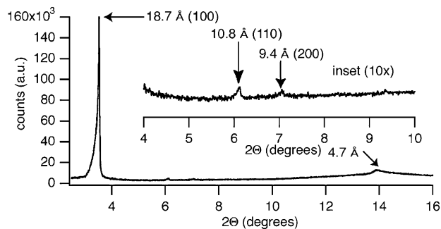
Figure 4. Synchrotron X-ray diffraction ( \lambda = 1.15 \text{ \AA} ) from a 2 mm Lindemann capillary tube filled with 1c at 150 °C.
