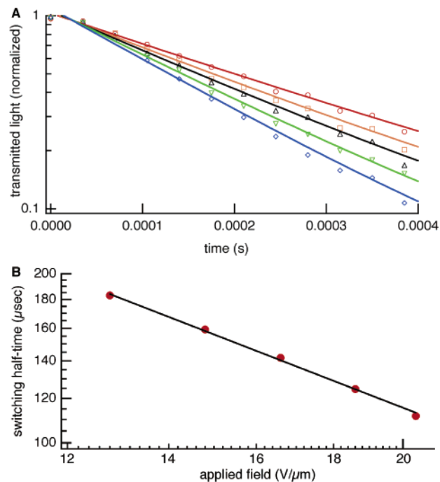
Figure 6. (a) Decrease in intensity of transmitted plane polarized light for 1c (150 ^{\circ}\text{C} ), as an electric field is triggered at t = 0 s, red = 12.8 \text{V}/\mu\text{m} , orange = 14.8 \text{V}/\mu\text{m} , black = 16.6 \text{V}/\mu\text{m} , green = 18.6 \text{V}/\mu\text{m} , blue = 20.4 \text{V}/\mu\text{m} ; the symbols are 1/50 of the measured data, and the color-coded solid lines are the curve fit. The y-axis is logarithmic. (b) A plot of the half-times for switching measured from Figure 6a versus the applied electric field. The axes are logarithmic. The solid line is a power function fit to the data.
