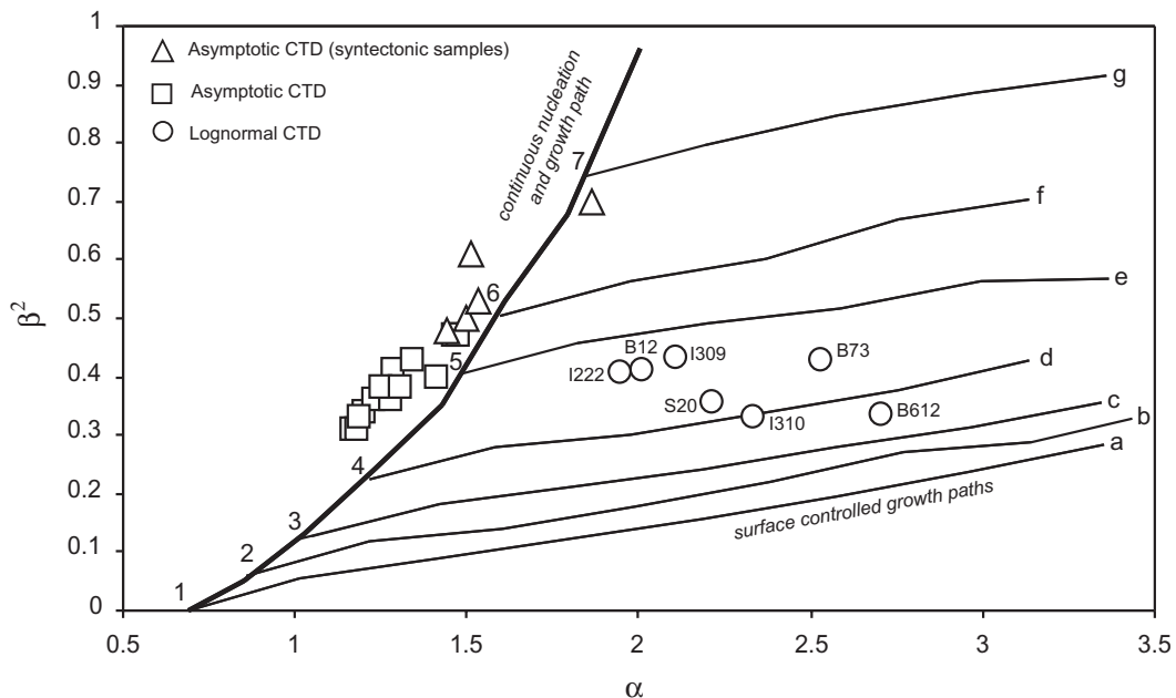
Fig. 2 \alpha vs \beta^2 diagram determined on the samples using the MudMaster program. 1–7, path for simultaneous, constant-rate nucleation and growth; a–g, paths for surface-controlled growth without simultaneous nucleation.
