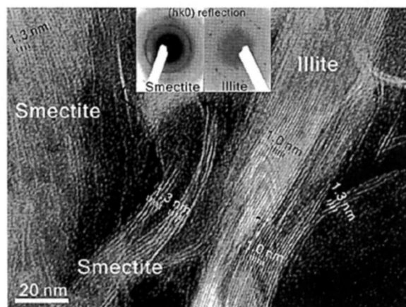
Fig. 2. TEM micrograph of the LR. White resin-embedded bioreduced smectite sample. Two phases of clay minerals were observed: An approximately 40-nm-thick packet of 1.0-nm illite layers occurred in the smectite matrix of 1.3-nm layers. The inset SAED patterns show the structural difference between these two phases in (hk0) reflections, in ring patterns (turbostratic typical of the smectite structure), and in discrete Bragg reflections (typical of the illite structure).
