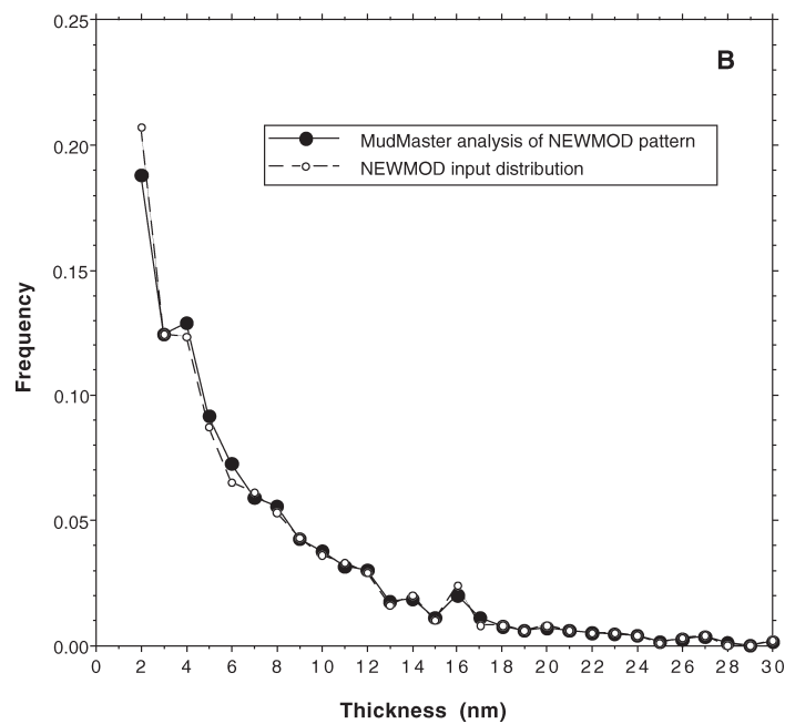
Fig. 1 (A) MudMaster analyses of a NEWMOD-calculated XRD pattern having a lognormal CTD with a mean thickness of 7 nm. An artifact appears at 2 nm for the non-smoothed CTD. (B) MudMaster analyzed CTD compared with CTD used as NEWMOD input. An artifact for the asymptotic CTD is not apparent at 2 nm.
