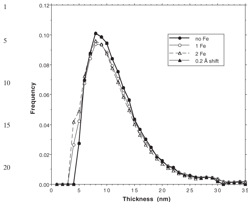
Fig. 4 Effect of various Fe contents and atomic positions used in calculation of the structure factor for crystallite size analysis of illite RM30 by MudMaster.
