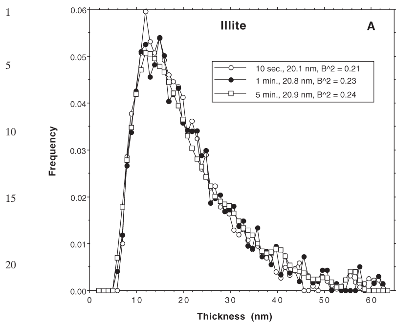
Fig. 7 Effect of ultrasonic probe treatment for various lengths of time on MudMaster-determined CTDs for (A) illite; (B) kaolinite; and (C) chlorite.
