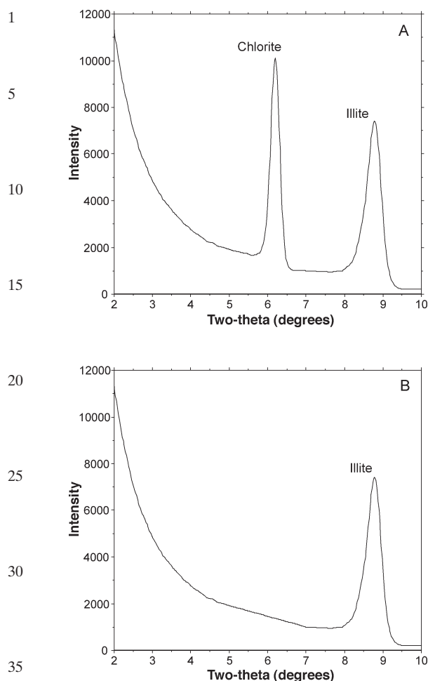
Fig. 2 (A) NEWMOD (Reynolds, 1985) calculated diffraction profiles for chlorite and illite mixed in the ratio 1:1. (B) Same pattern as in A, but the chlorite peak has been removed using PeakChopper.
