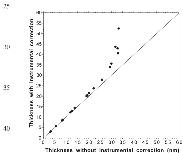
Fig. 5 Effect of instrumental broadening correction as a function of crystallite size for illites from the Glarus Alps (samples from Hunziker et al., 1986).
